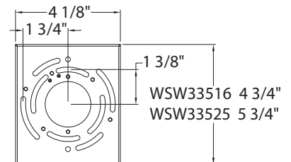
Mounting Plate Dimensions
